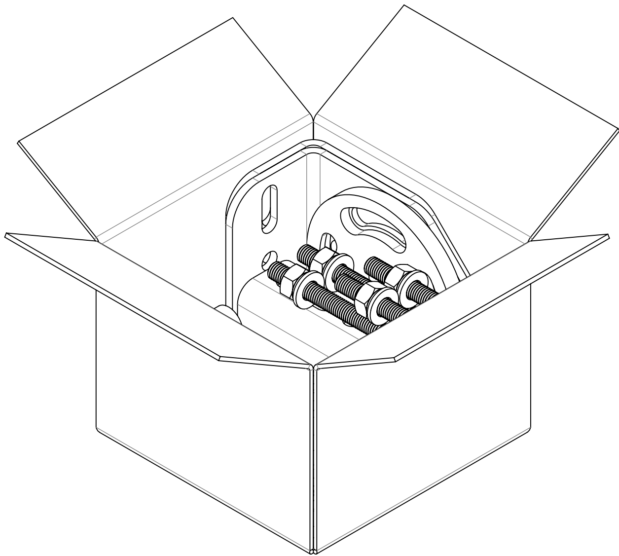
PACKAGING VIEW
